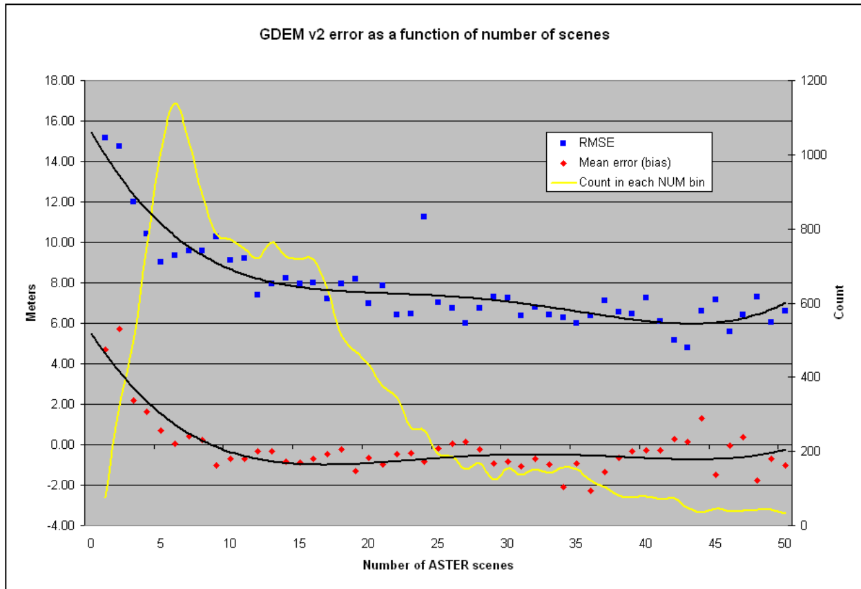
Figure 2 The relationship between mean and RMS error, and the stacking number (“NUM”), using 18,000 geodetic control points as a reference over the Conterminous U.S. The yellow line indicates the number of pixels having a given stacking number value; thus “NUM” values below 3 or above 23 occur rarely in this region. Note that the occurrence of low “NUM” values can be more common over persistently cloudy regions, particularly at high latitudes.
